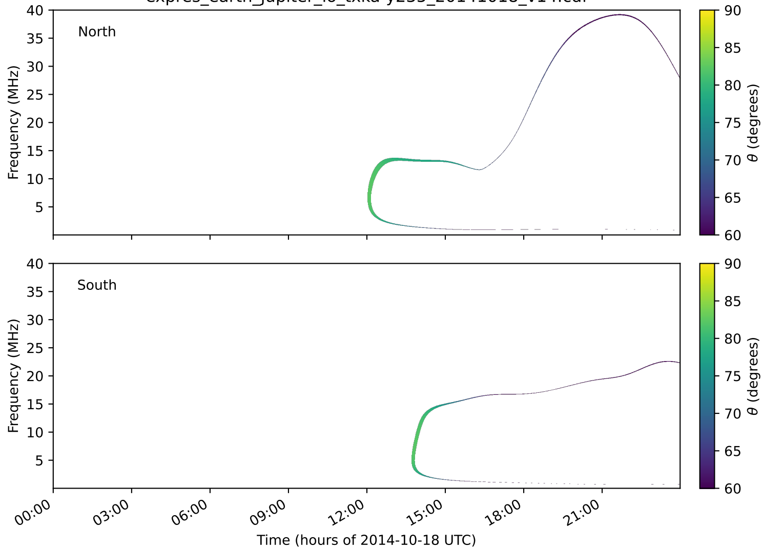
expres_earth_jupiter_io_txka-y235_20141018_v14.cdf
