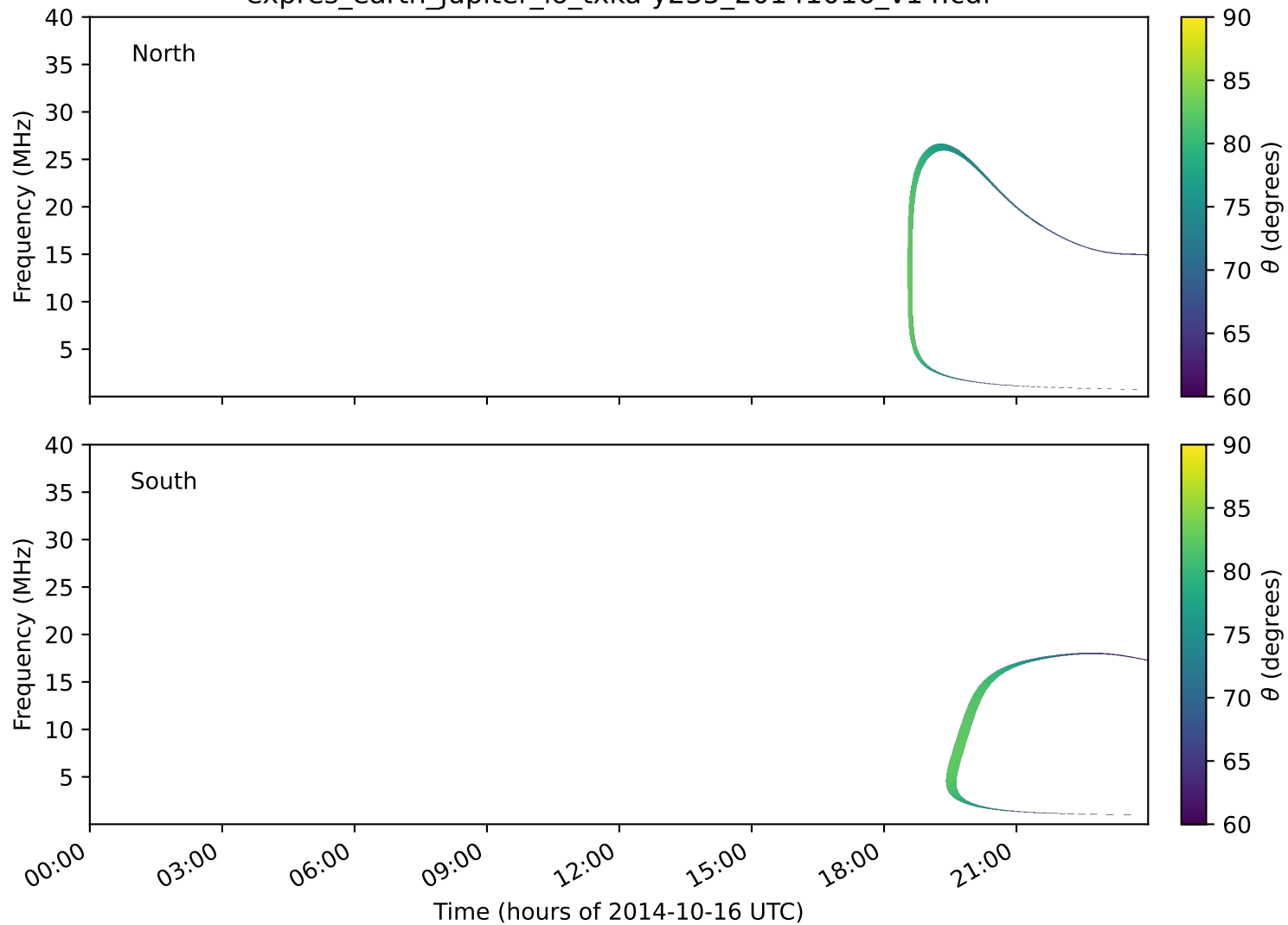
expres_earth_jupiter_io_txka-y235_20141016_v14.cdf
