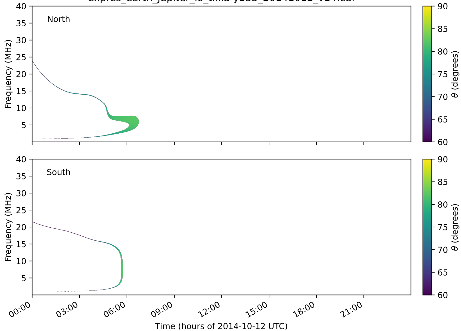
expres_earth_jupiter_io_txka-y235_20141012_v14.cdf
