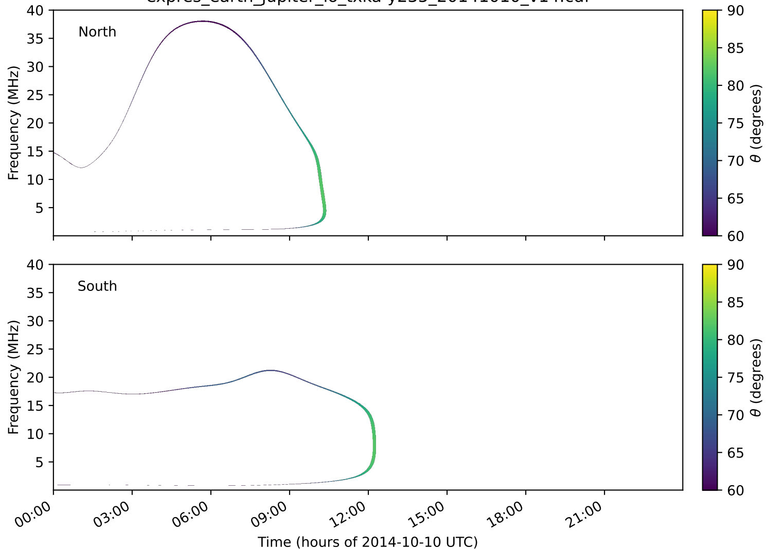
expres_earth_jupiter_io_txka-y235_20141010_v14.cdf
