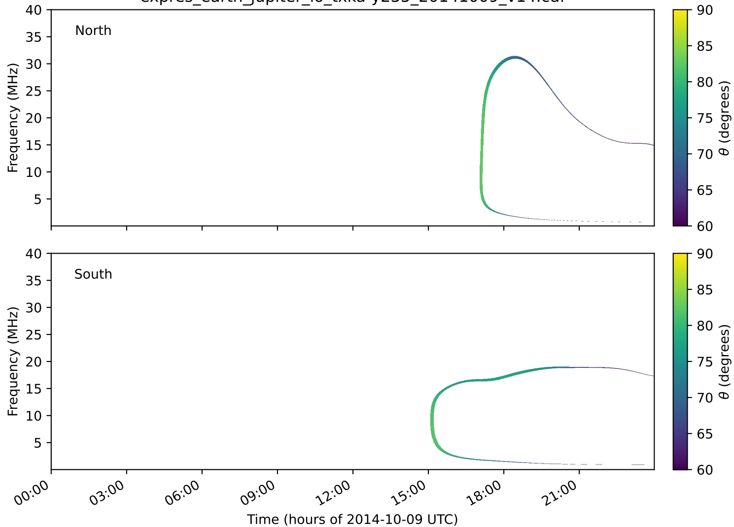
expres_earth_jupiter_io_txka-y235_20141009_v14.cdf
