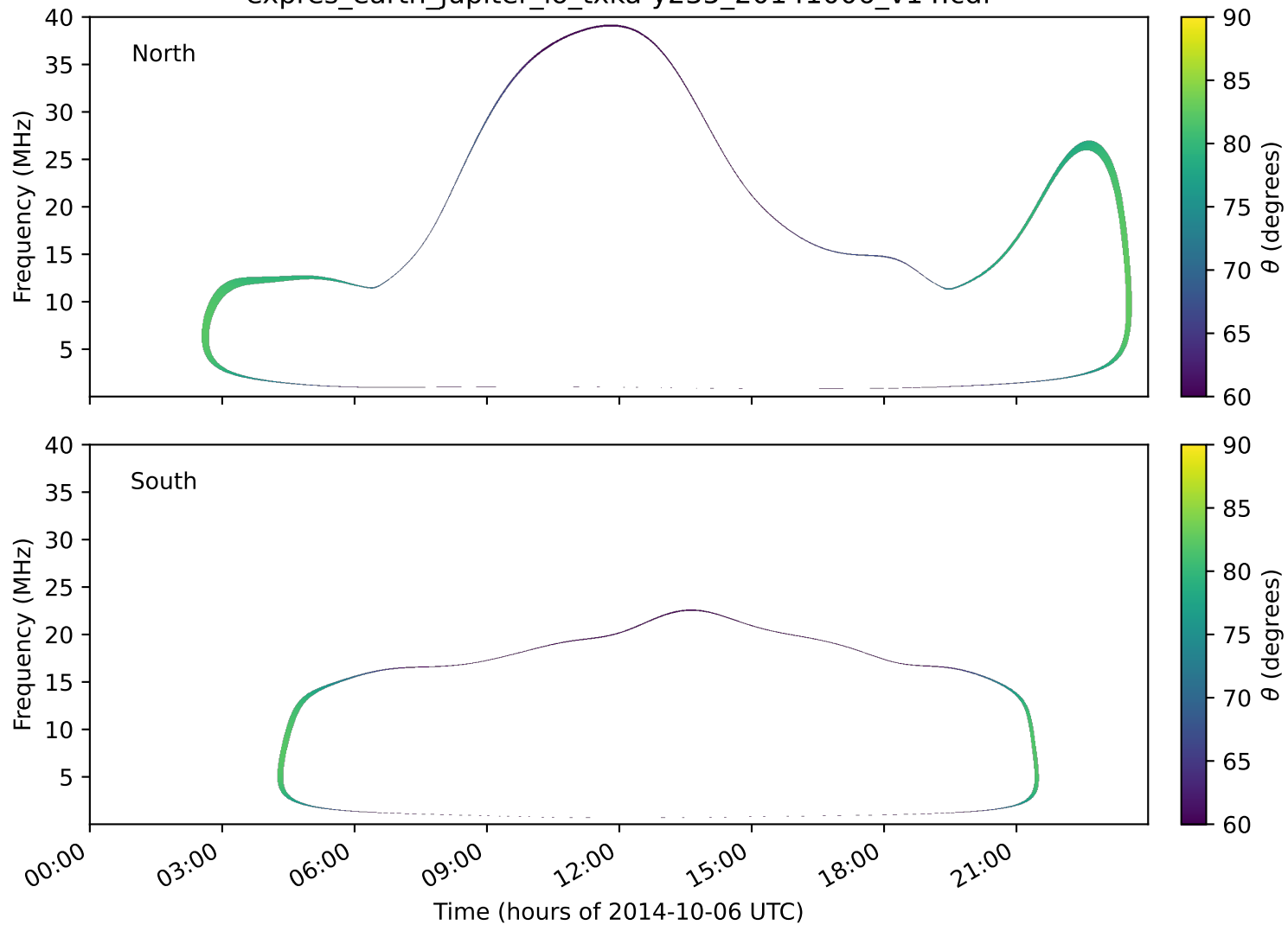
expres_earth_jupiter_io_txka-y235_20141006_v14.cdf
