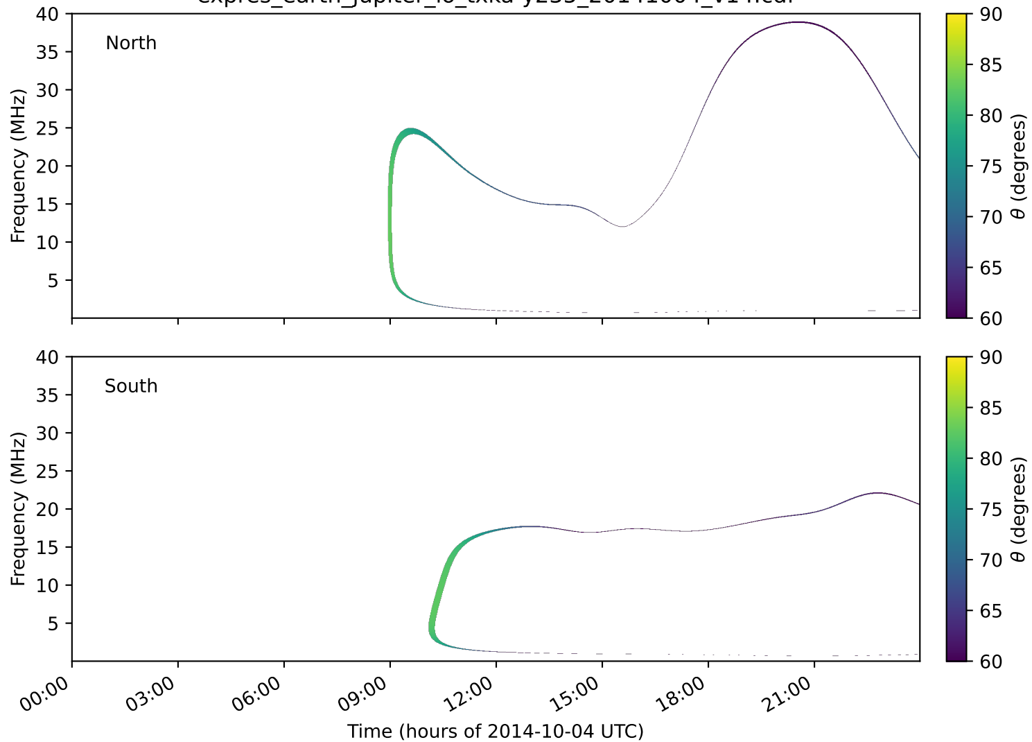
expres_earth_jupiter_io_txka-y235_20141004_v14.cdf
