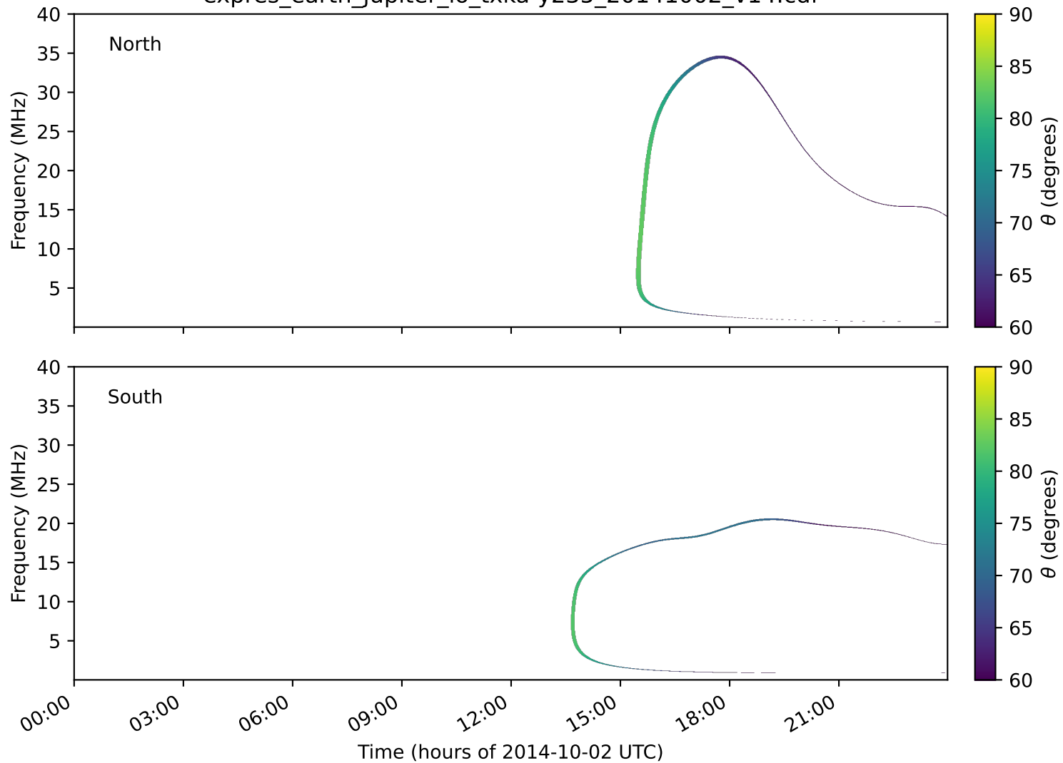
expres_earth_jupiter_io_txka-y235_20141002_v14.cdf
