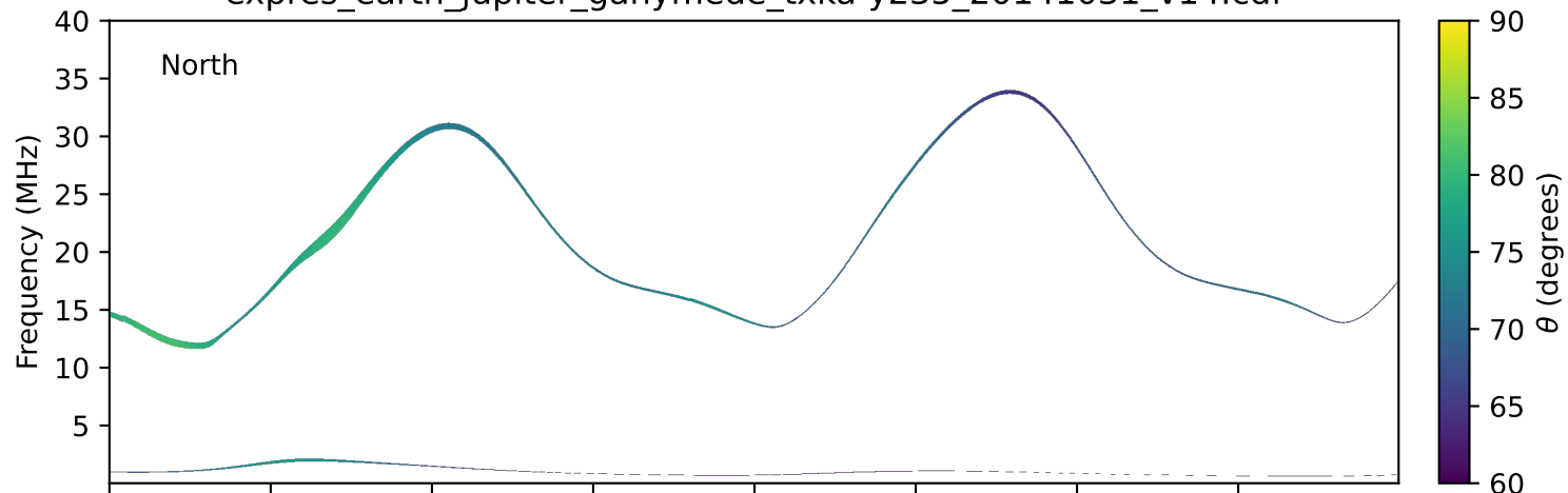
expres_earth_jupiter_ganymede_txka-y235_20141031_v14.cdf
