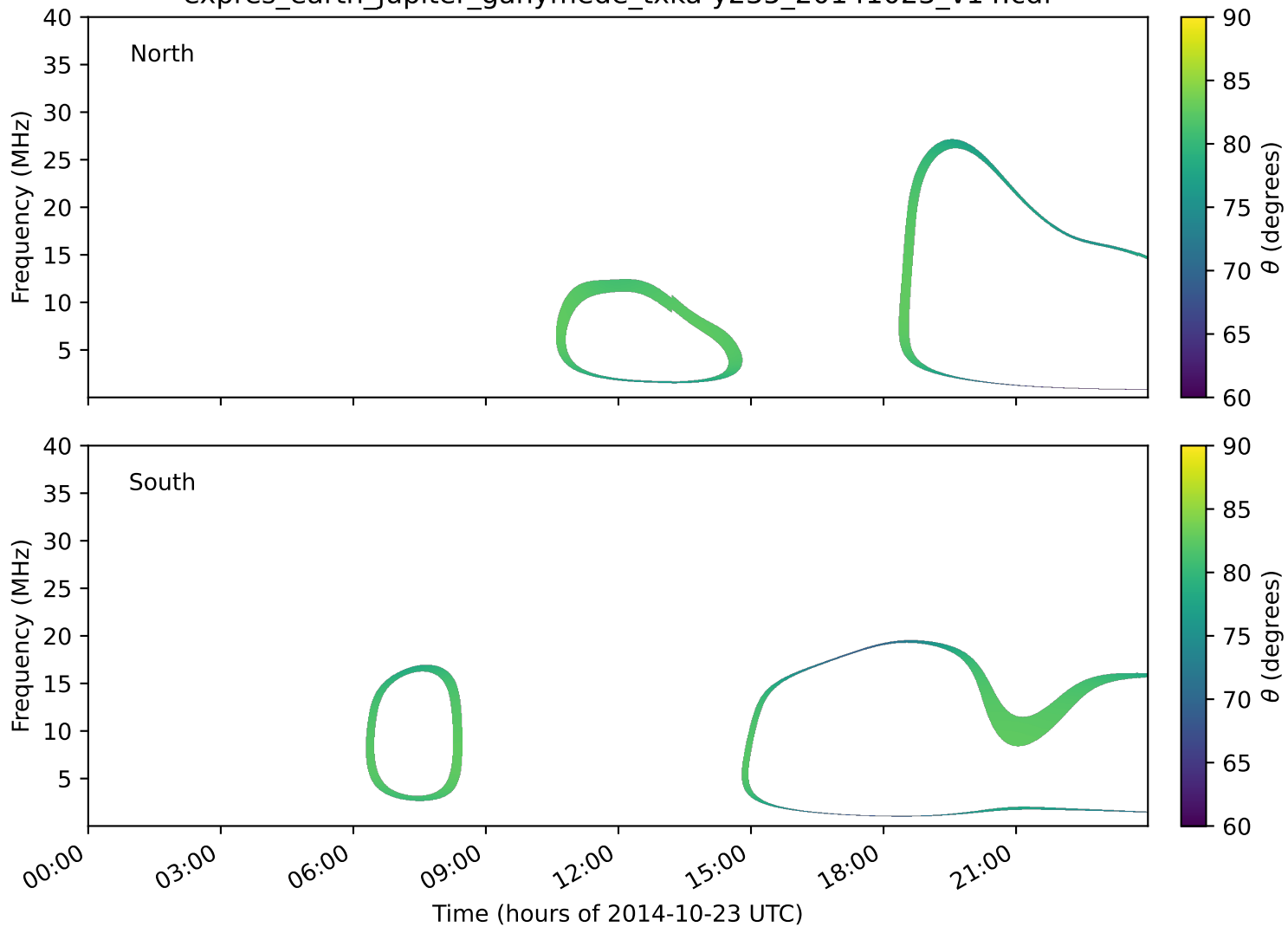
expres_earth_jupiter_ganymede_txka-y235_20141023_v14.cdf
