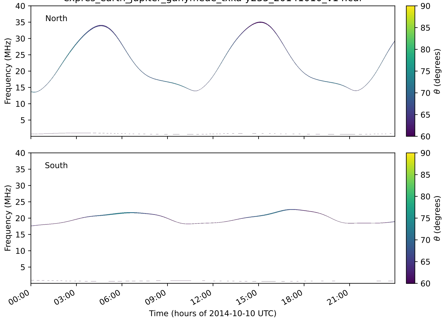
expres_earth_jupiter_ganymede_txka-y235_20141010_v14.cdf
