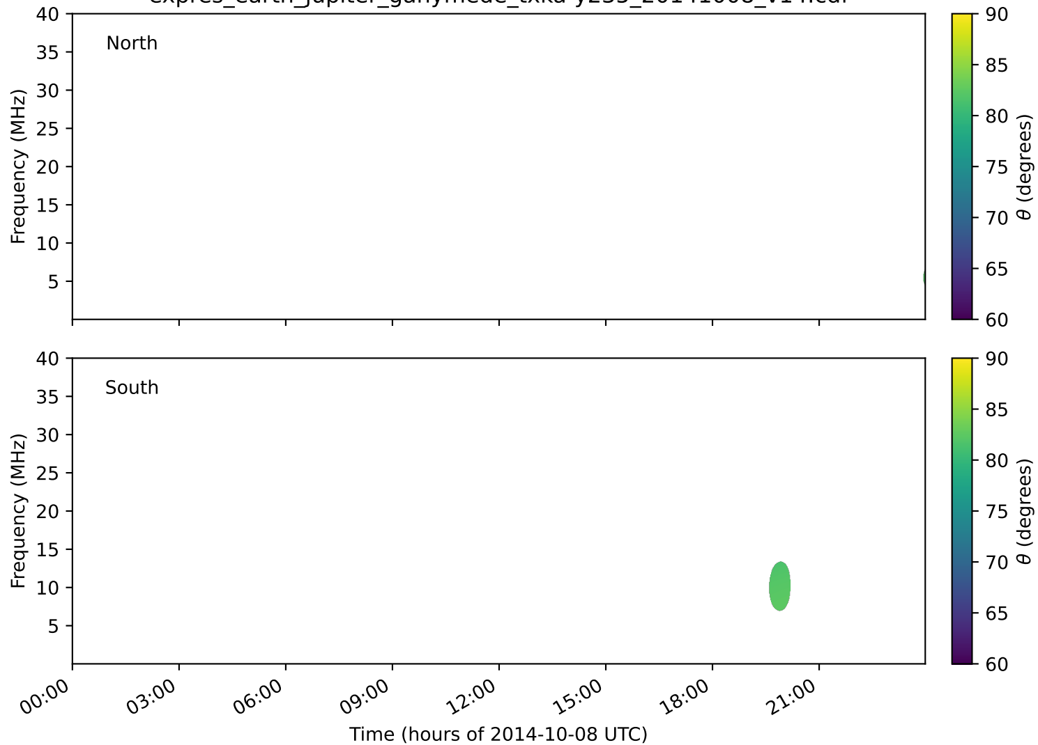
expres_earth_jupiter_ganymede_txka-y235_20141008_v14.cdf
