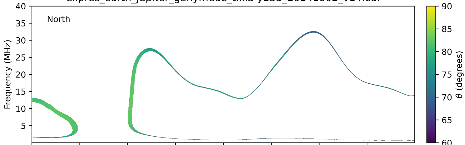
expres_earth_jupiter_ganymede_txka-y235_20141002_v14.cdf
