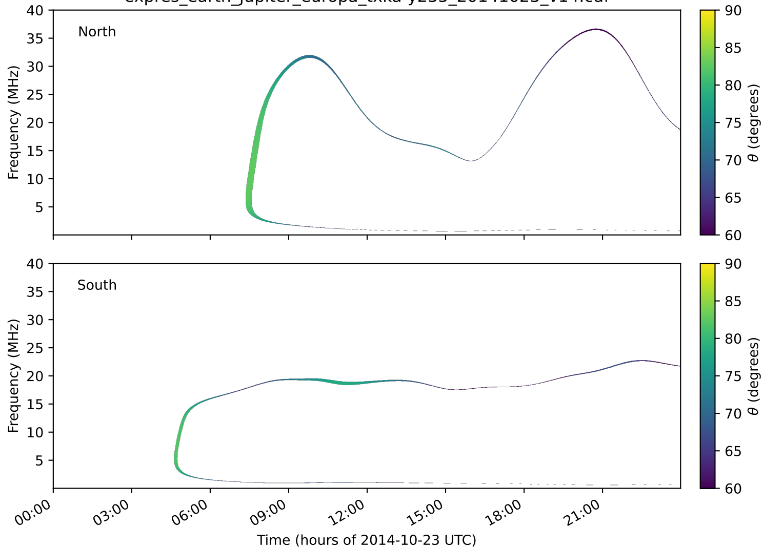
expres_earth_jupiter_europa_txka-y235_20141023_v14.cdf
