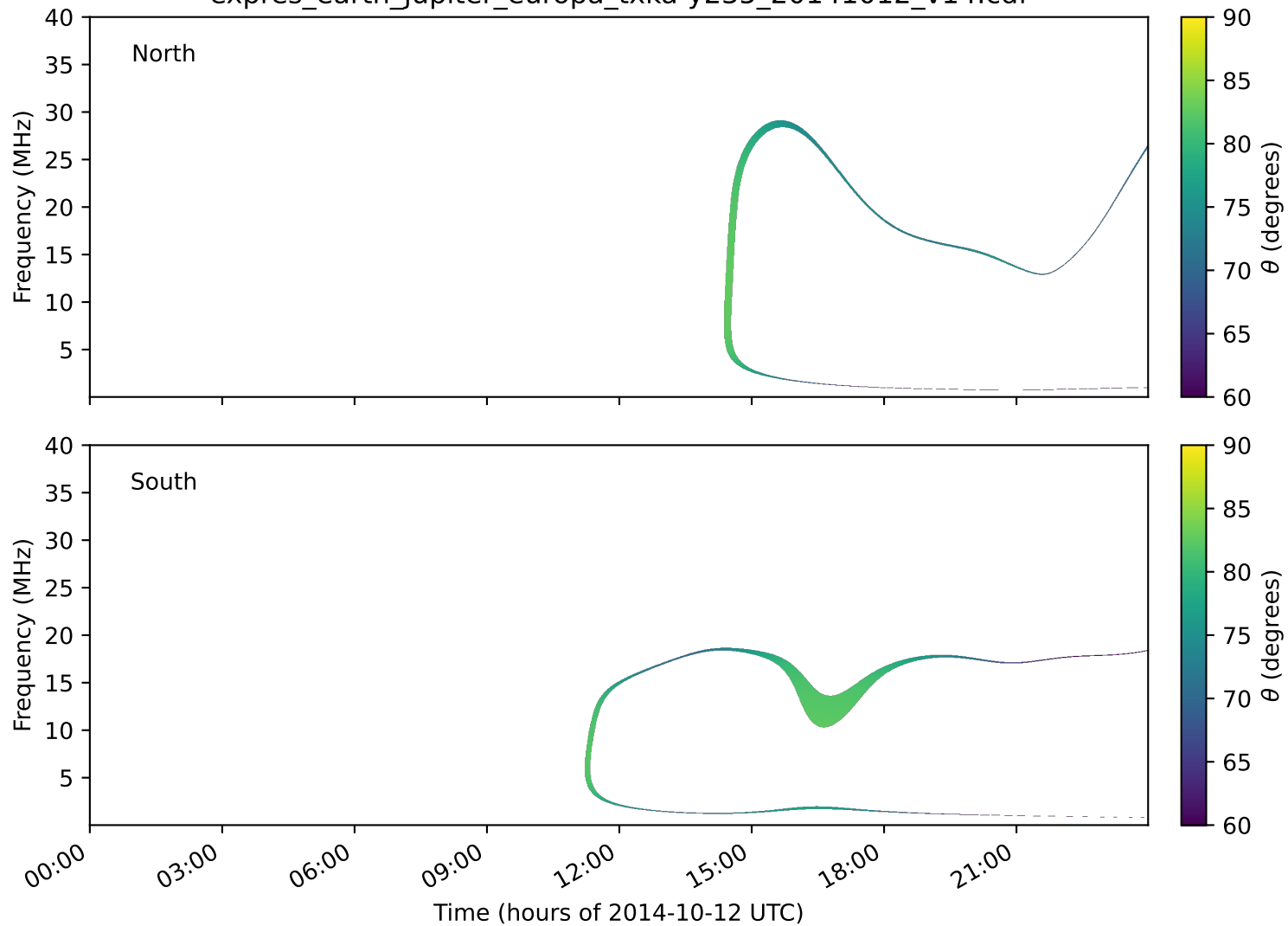
expres_earth_jupiter_europa_txka-y235_20141012_v14.cdf
