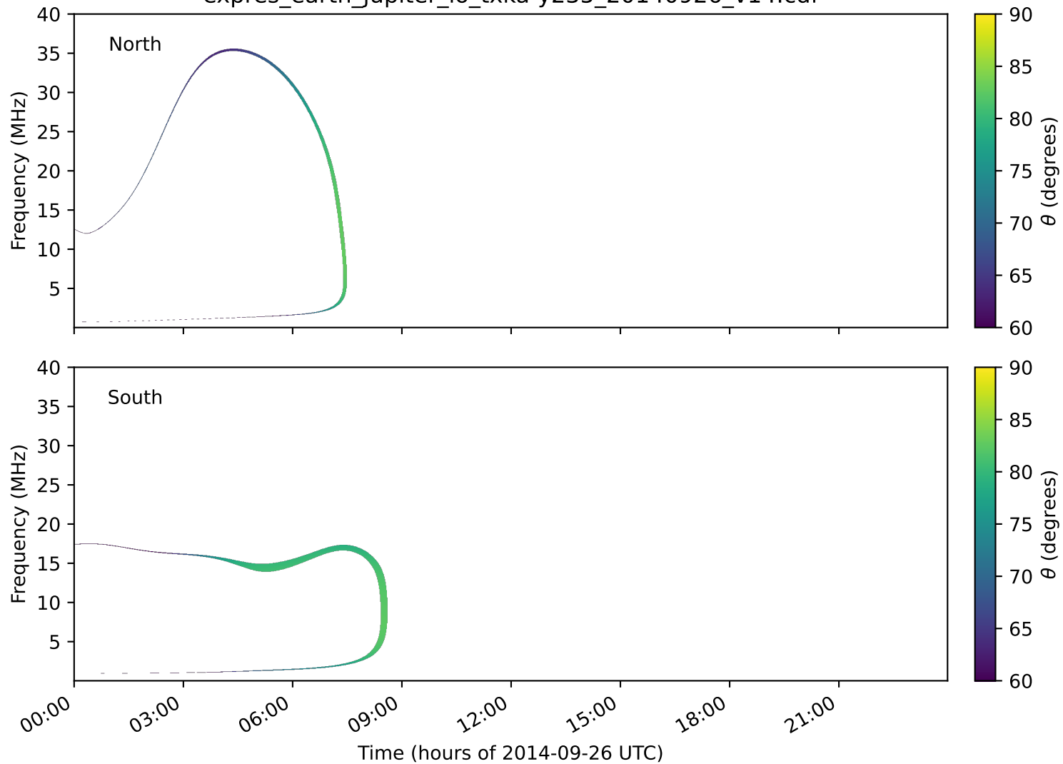
expres_earth_jupiter_io_txka-y235_20140926_v14.cdf
