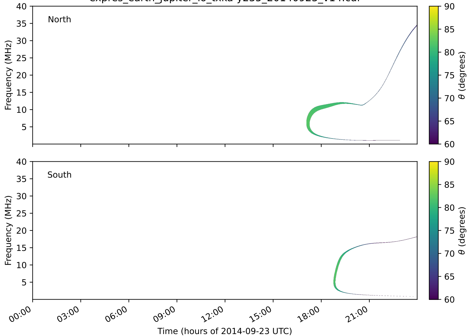
expres_earth_jupiter_io_txka-y235_20140923_v14.cdf
