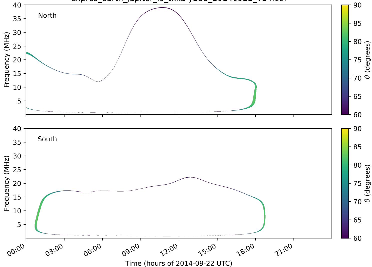
expres_earth_jupiter_io_txka-y235_20140922_v14.cdf
