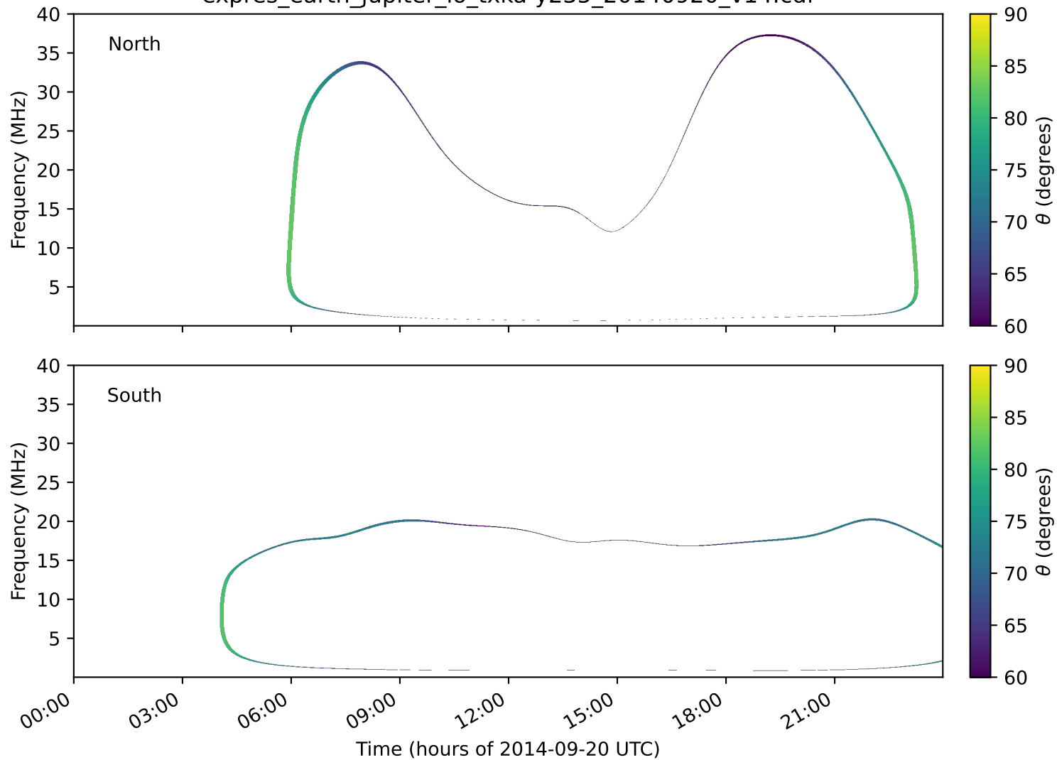
expres_earth_jupiter_io_txka-y235_20140920_v14.cdf
