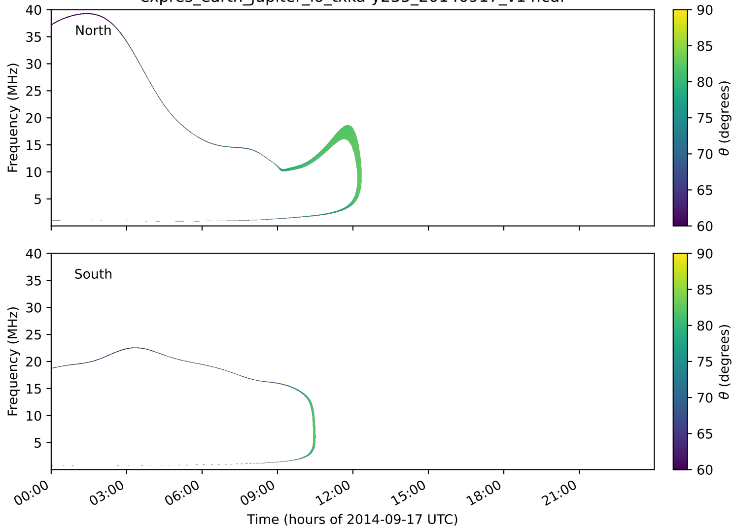
expres_earth_jupiter_io_txka-y235_20140917_v14.cdf
