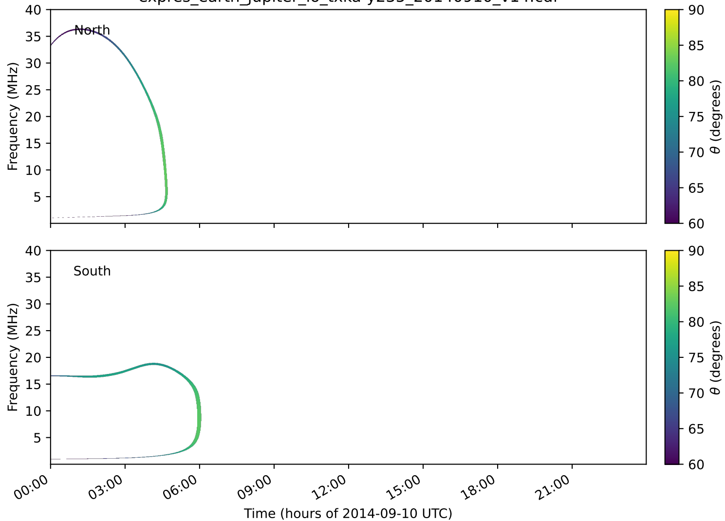
expres_earth_jupiter_io_txka-y235_20140910_v14.cdf
