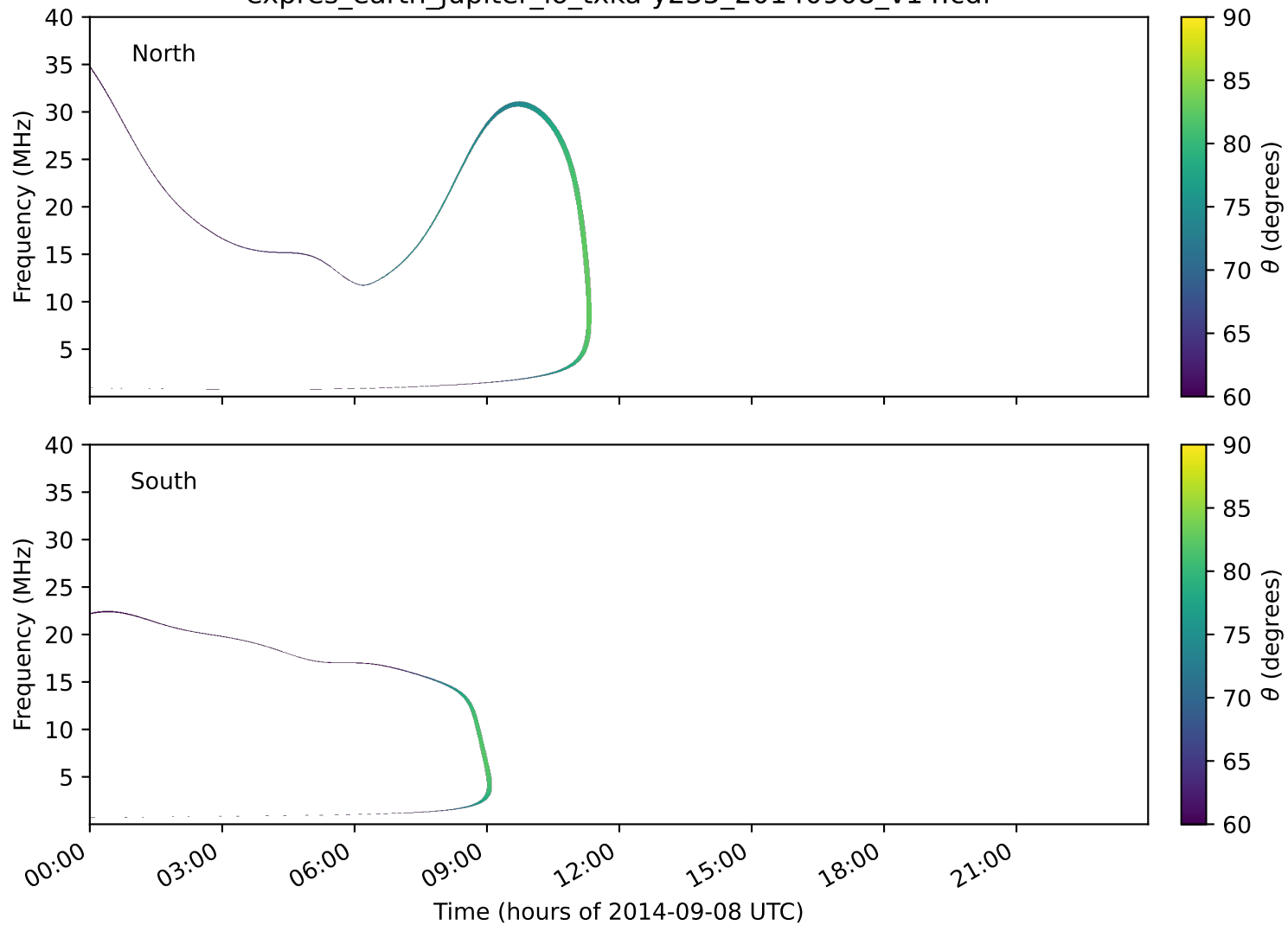
expres_earth_jupiter_io_txka-y235_20140908_v14.cdf
