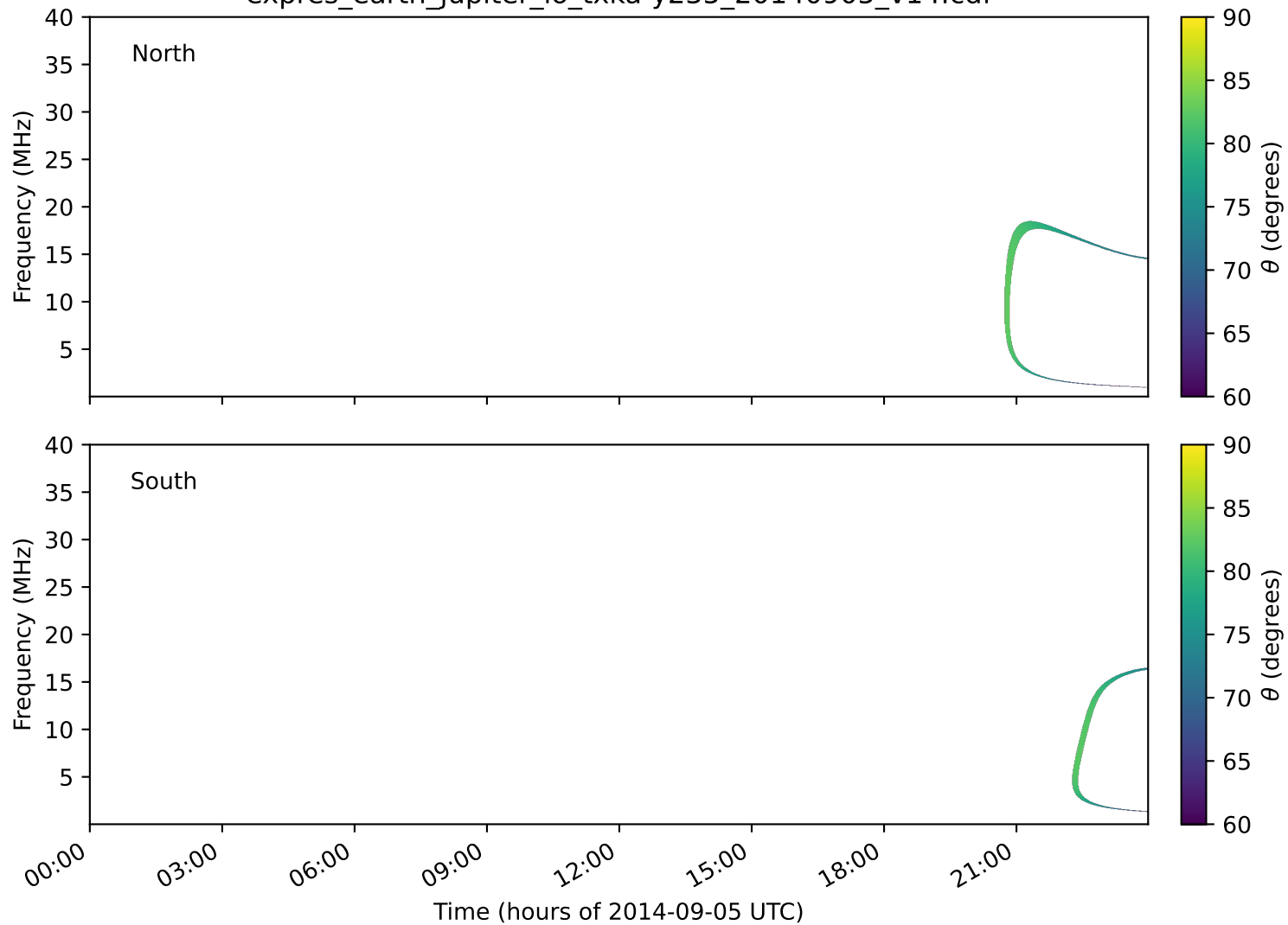
expres_earth_jupiter_io_txka-y235_20140905_v14.cdf
