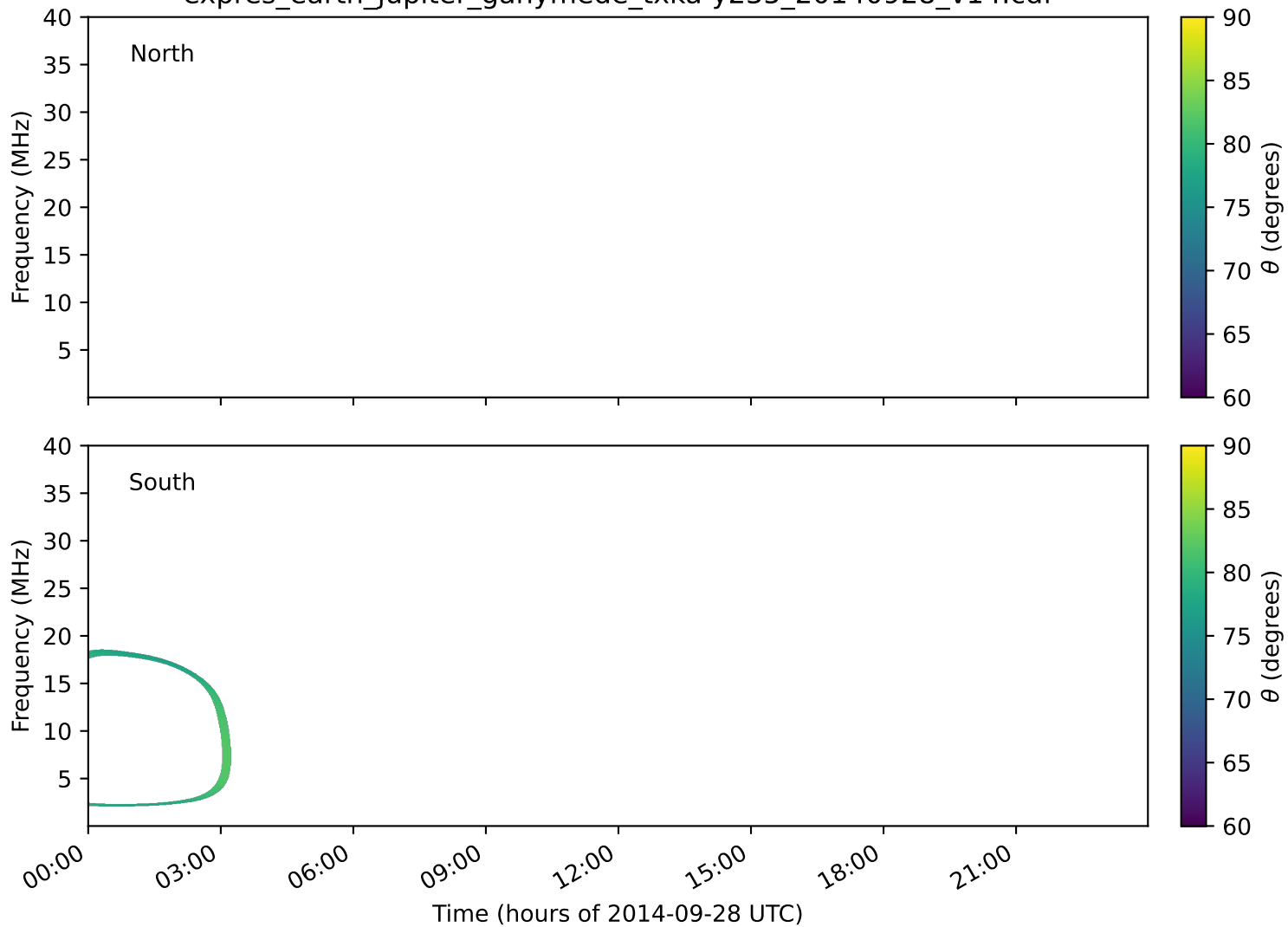
expres_earth_jupiter_ganymede_txka-y235_20140928_v14.cdf
