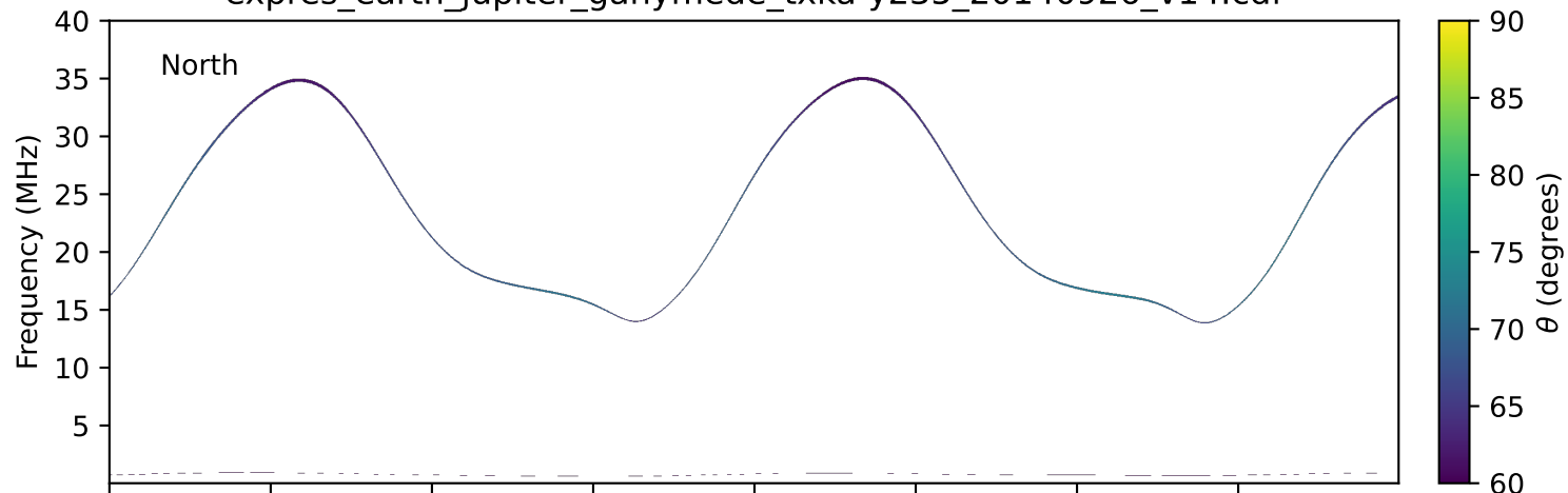
expres_earth_jupiter_ganymede_txka-y235_20140926_v14.cdf
