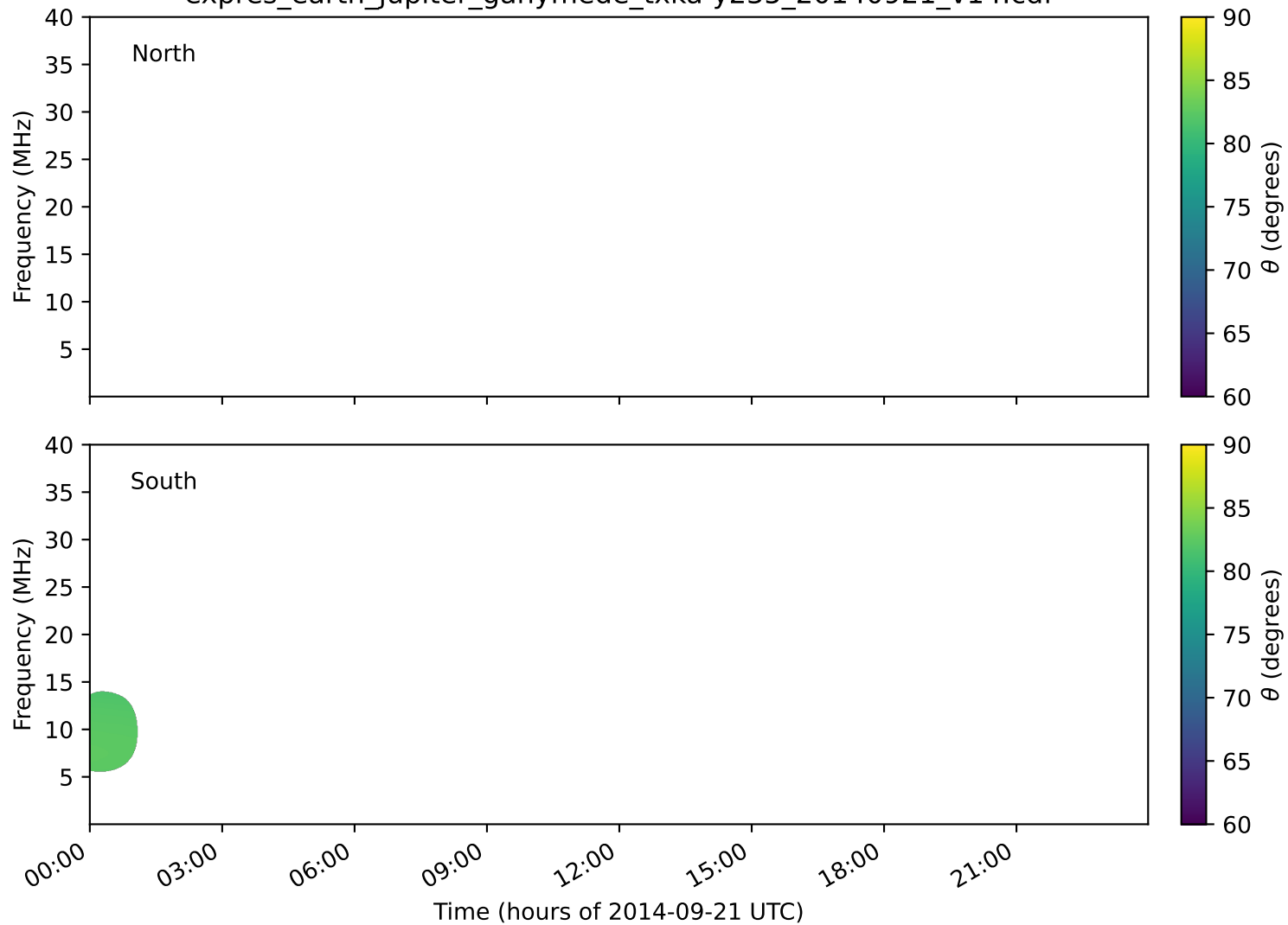
expres_earth_jupiter_ganymede_txka-y235_20140921_v14.cdf
