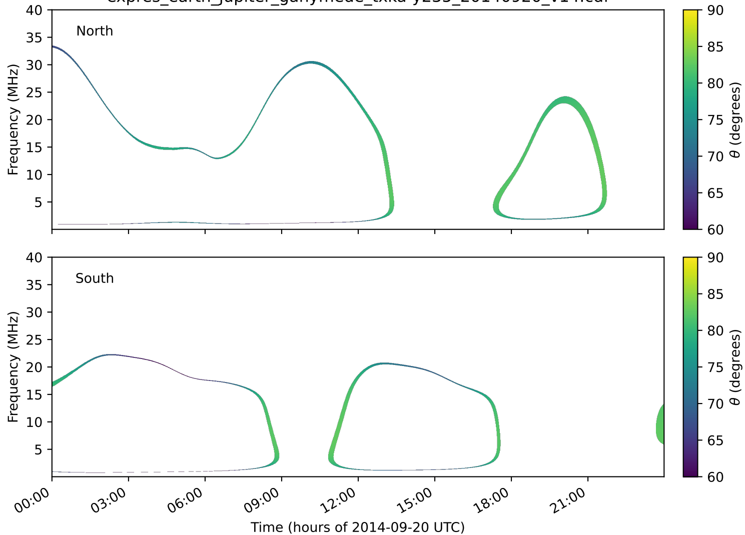
expres_earth_jupiter_ganymede_txka-y235_20140920_v14.cdf
