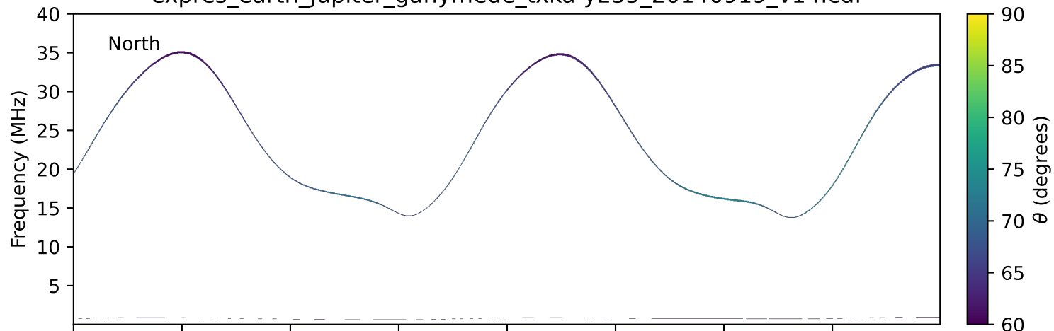
expres_earth_jupiter_ganymede_txka-y235_20140919_v14.cdf
