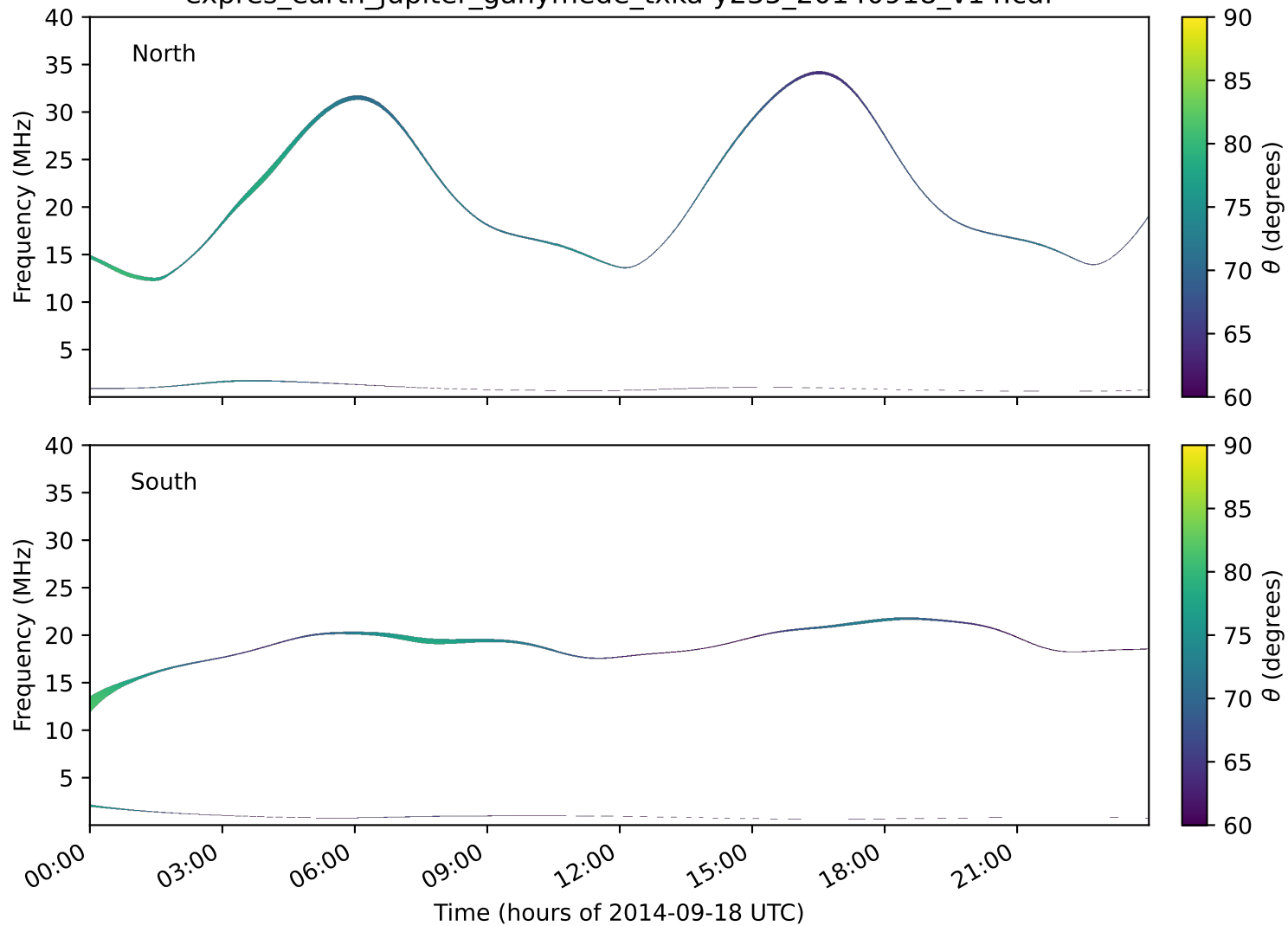
expres_earth_jupiter_ganymede_txka-y235_20140918_v14.cdf
