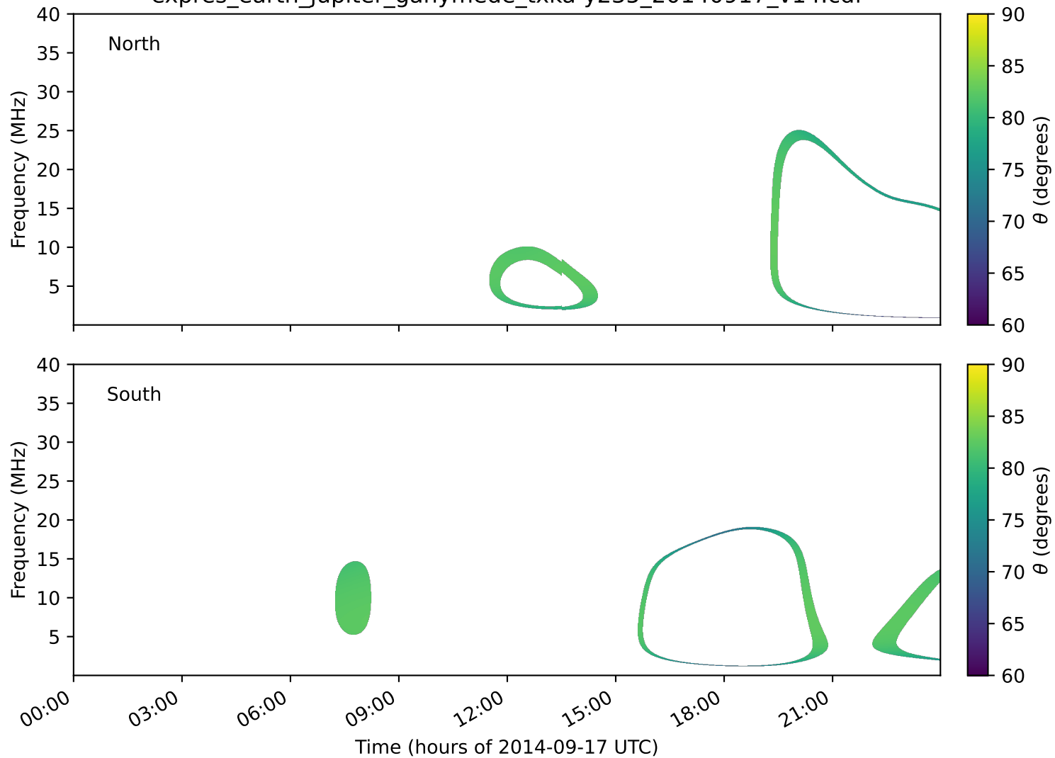
expres_earth_jupiter_ganymede_txka-y235_20140917_v14.cdf
