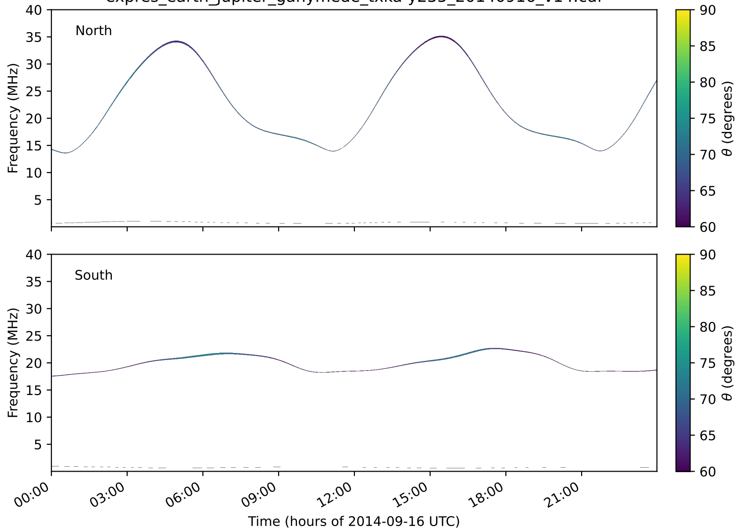
expres_earth_jupiter_ganymede_txka-y235_20140916_v14.cdf
