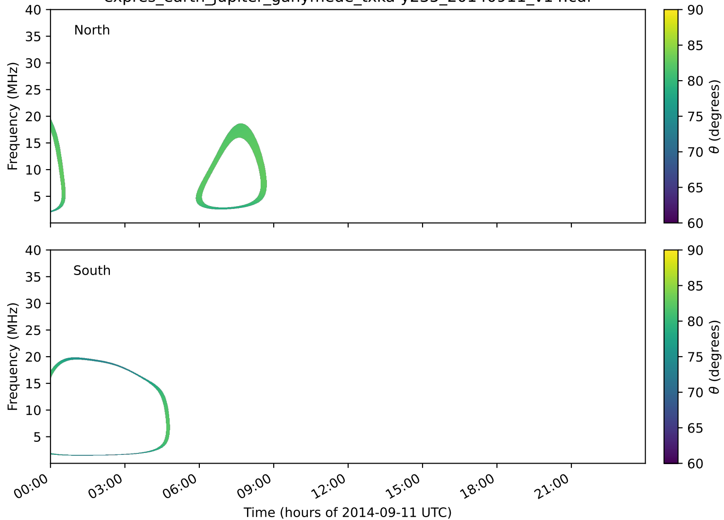
expres_earth_jupiter_ganymede_txka-y235_20140911_v14.cdf
