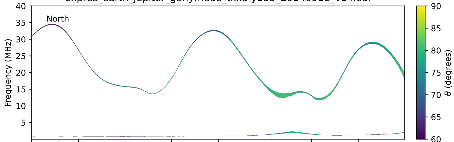
expres_earth_jupiter_ganymede_txka-y235_20140910_v14.cdf
