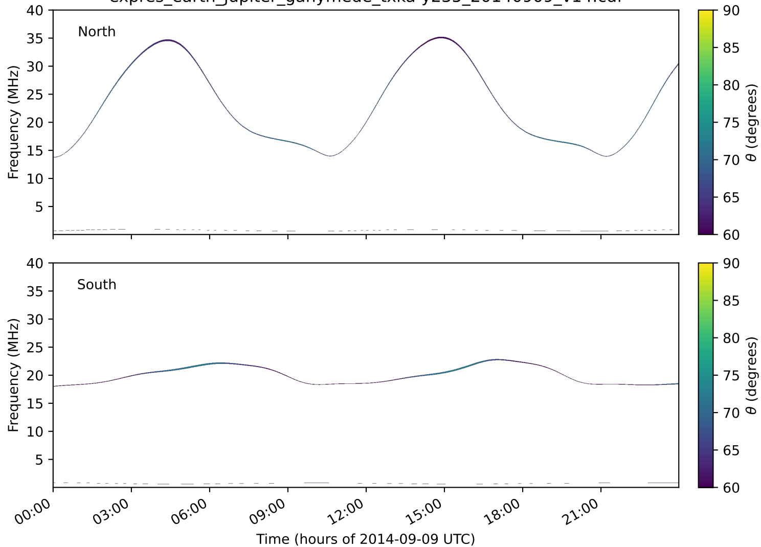
expres_earth_jupiter_ganymede_txka-y235_20140909_v14.cdf
