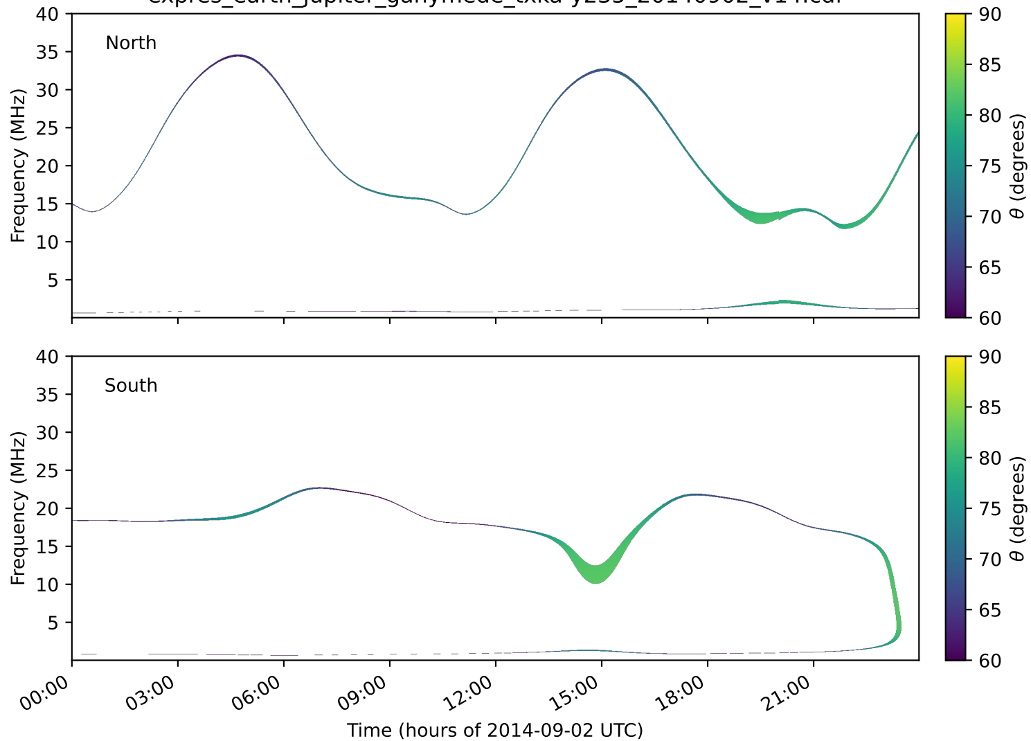
expres_earth_jupiter_ganymede_txka-y235_20140902_v14.cdf
