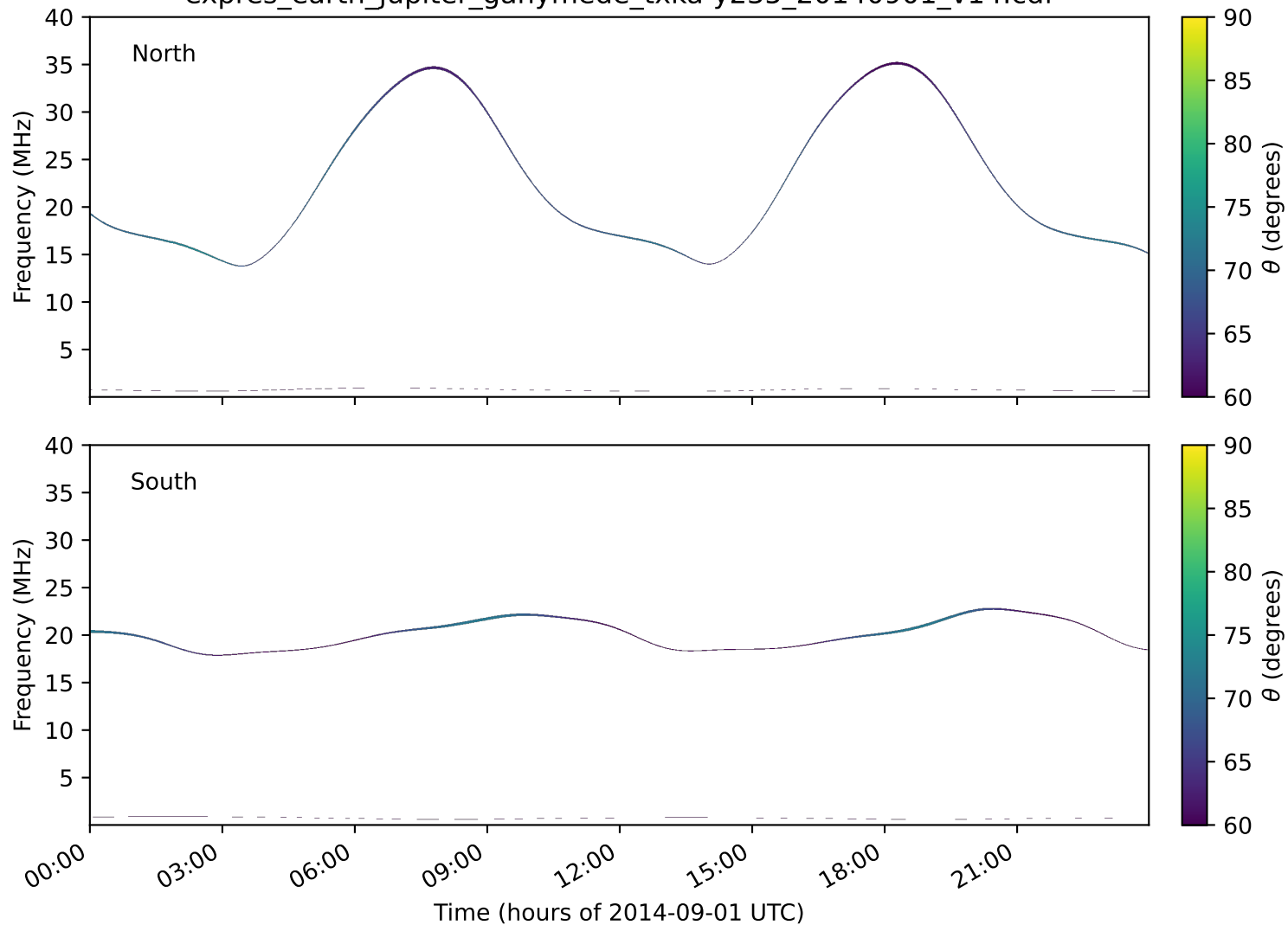
expres_earth_jupiter_ganymede_txka-y235_20140901_v14.cdf
