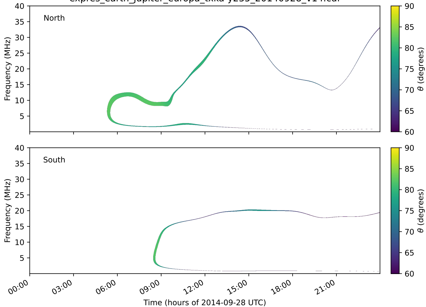
expres_earth_jupiter_europa_txka-y235_20140928_v14.cdf
