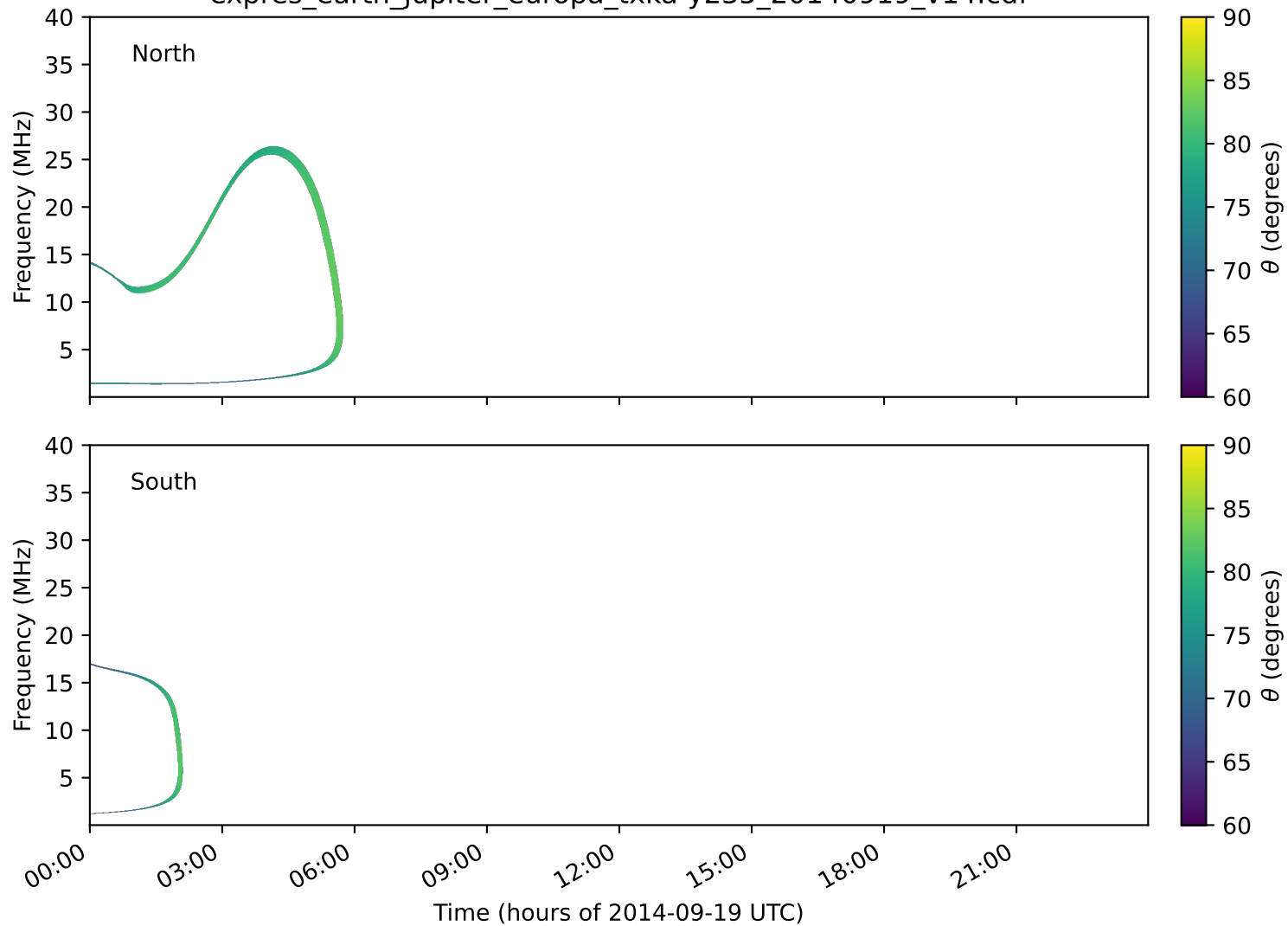
expres_earth_jupiter_europa_txka-y235_20140919_v14.cdf
