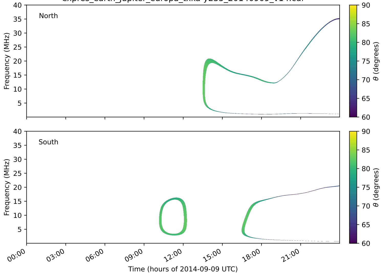
expres_earth_jupiter_europa_txka-y235_20140909_v14.cdf
