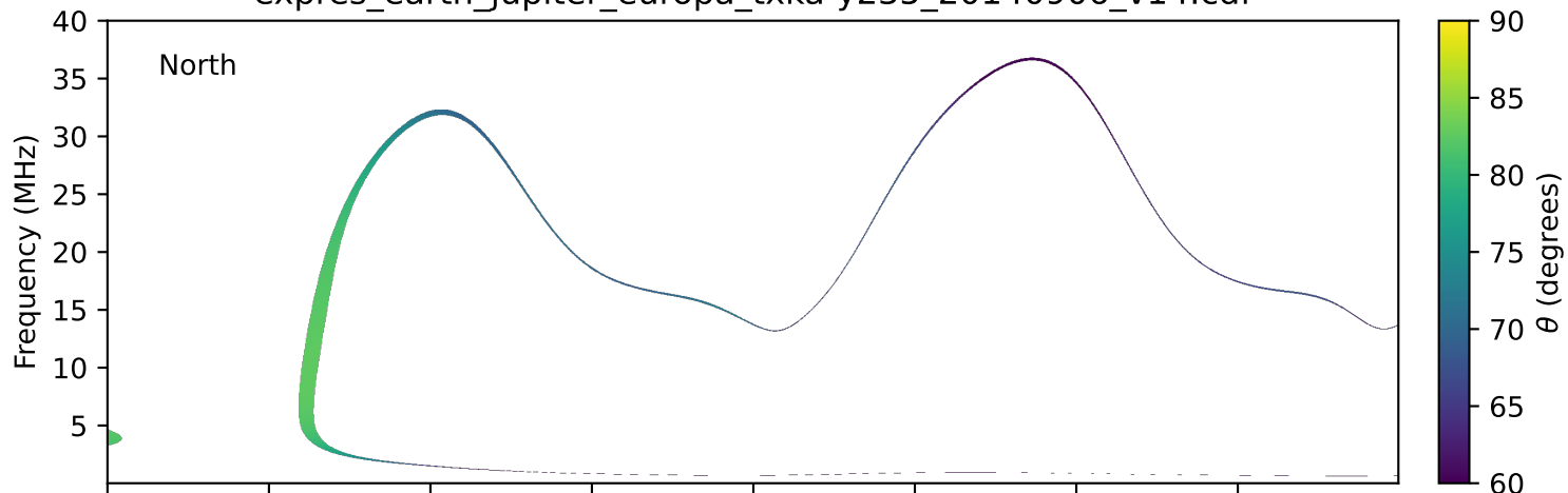
expres_earth_jupiter_europa_txka-y235_20140906_v14.cdf
