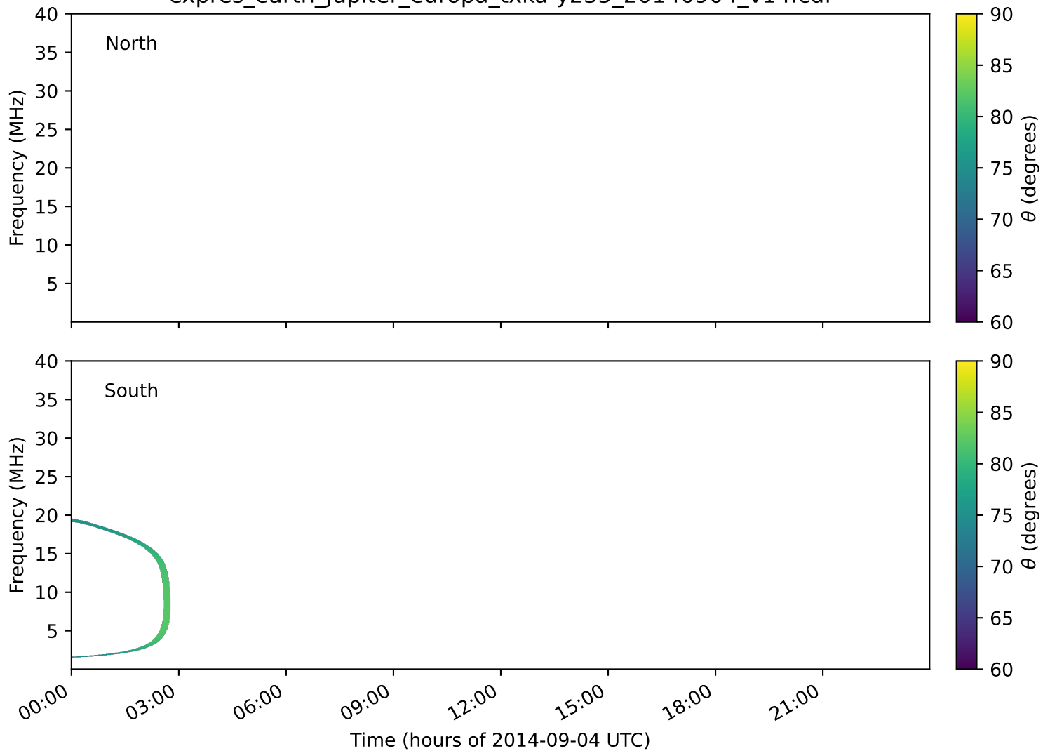
expres_earth_jupiter_europa_txka-y235_20140904_v14.cdf
