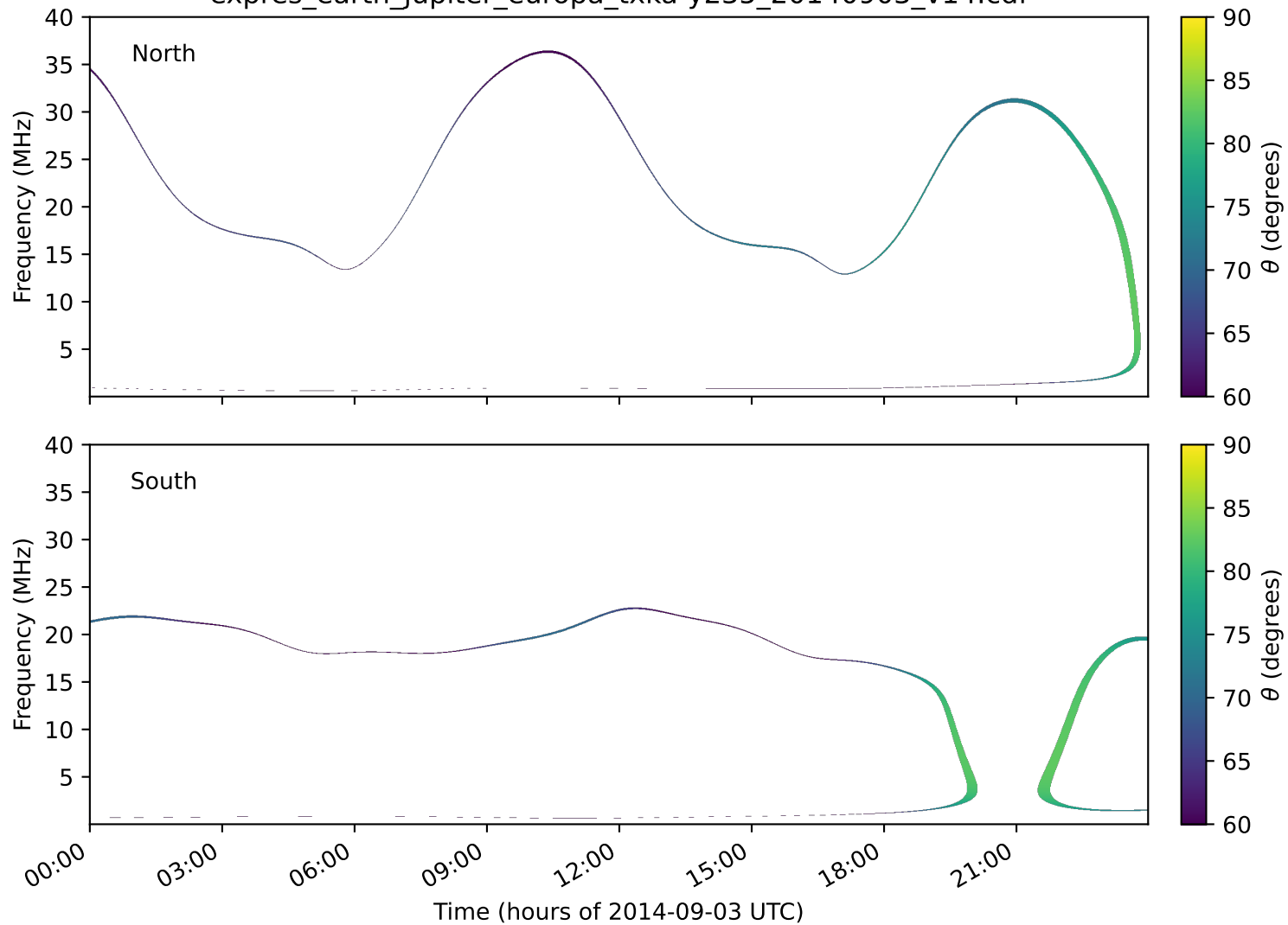
expres_earth_jupiter_europa_txka-y235_20140903_v14.cdf
