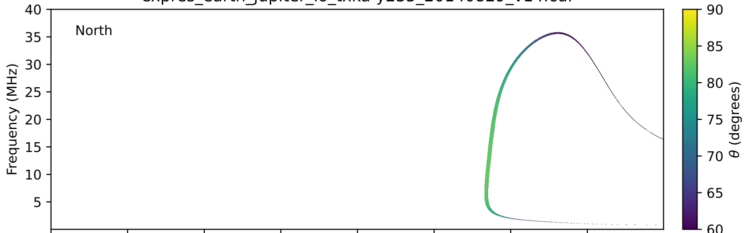
expres_earth_jupiter_io_txka-y235_20140829_v14.cdf
