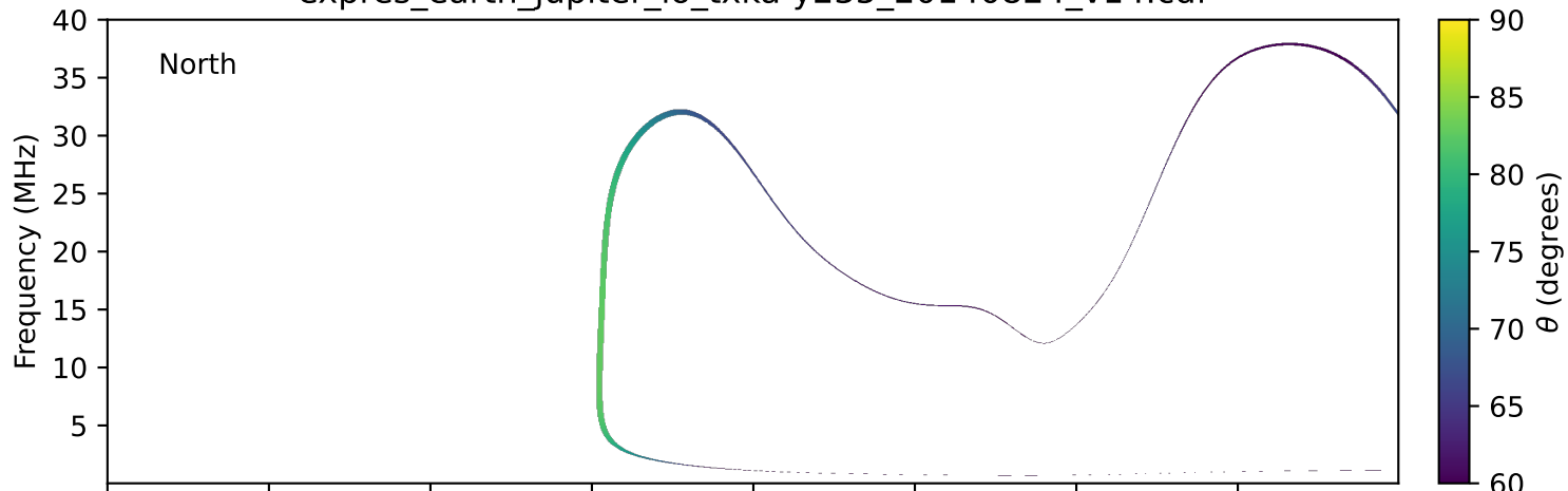
expres_earth_jupiter_io_txka-y235_20140824_v14.cdf
