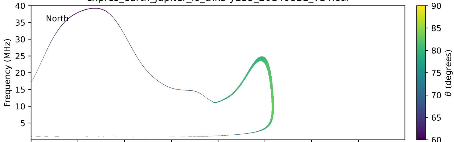
expres_earth_jupiter_io_txka-y235_20140821_v14.cdf
