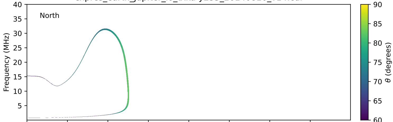
expres_earth_jupiter_io_txka-y235_20140816_v14.cdf
