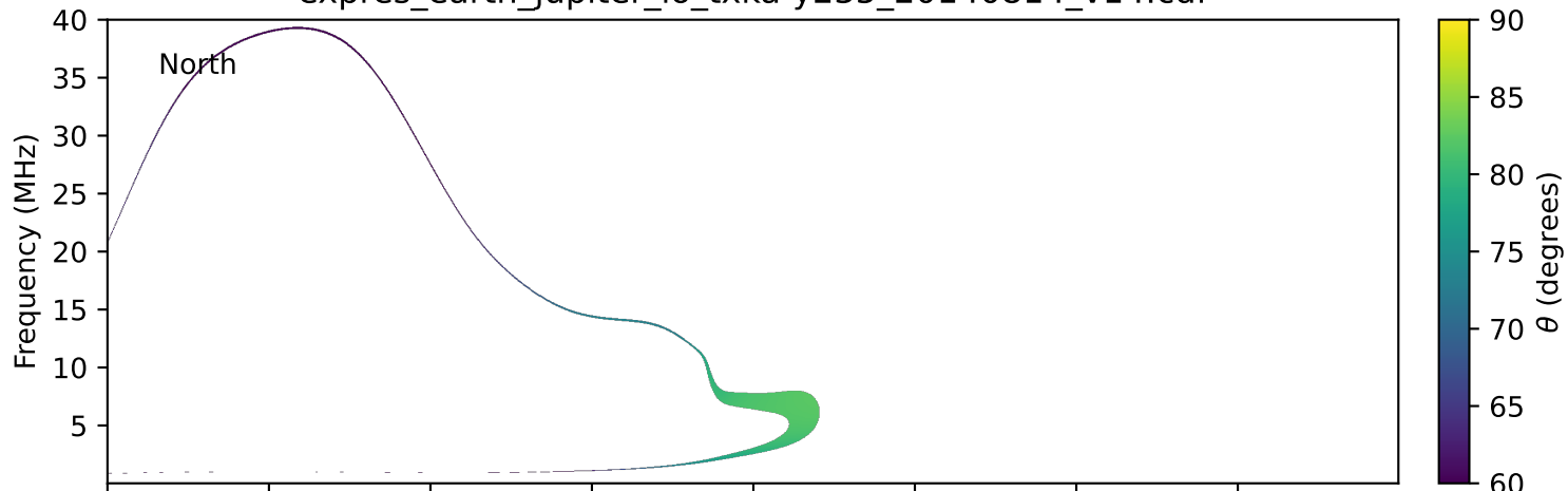
expres_earth_jupiter_io_txka-y235_20140814_v14.cdf
