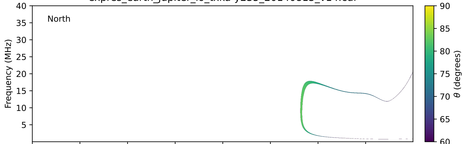
expres_earth_jupiter_io_txka-y235_20140813_v14.cdf
