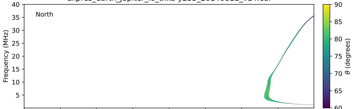
expres_earth_jupiter_io_txka-y235_20140811_v14.cdf
