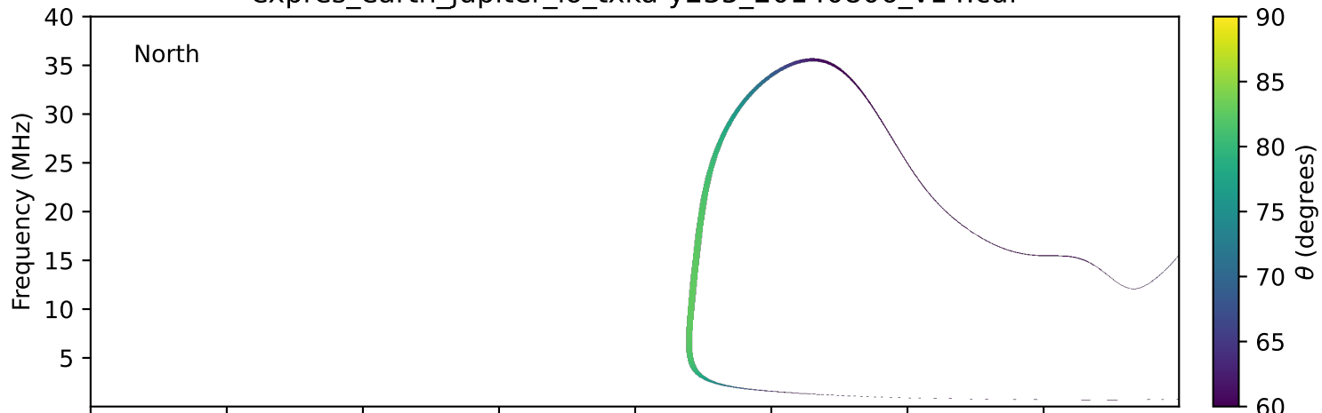
expres_earth_jupiter_io_txka-y235_20140806_v14.cdf
